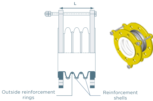
BELLOW STANDARD RANGE G227 3 convolutions only
