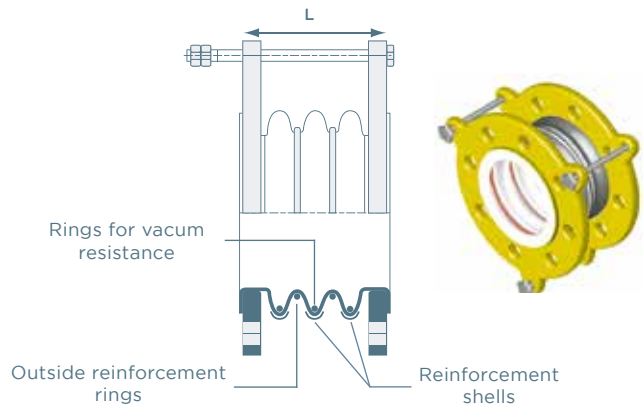
BELLOW RANGE VACUUM V227 3 convolutions only
